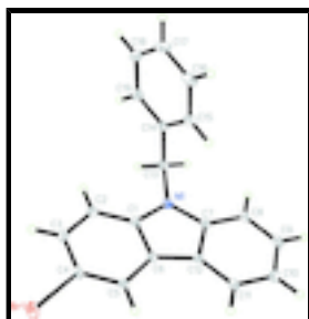
Fig. 1. Molecular structure of (I) with displacement ellipsoids drawn at the 30% probability level. H atoms are presented as spheres of arbitrary radius.
